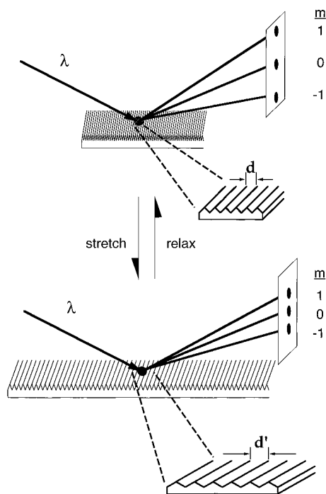
Figure 1. Stretching an elastomeric diffraction grating changes the periodicity of the grating and alters the spacing of the diffraction pattern. Features are not drawn to scale.
