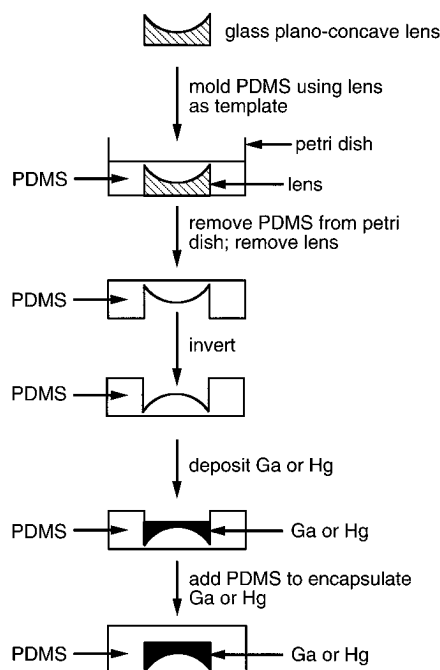
Figure 3. Schematic of the procedure for the fabrication of deformable mirrors. Features are not drawn to scale. See text for details.
