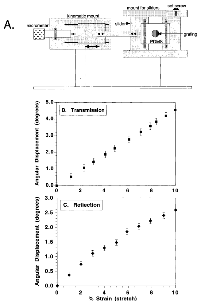
Figure 5. (a) Schematic of the homebuilt jig used to test the performance of elastomeric gratings and mirrors. The grating or mirror was mounted on two aluminum sliders held in an aluminum mount. One slider was fixed in place with a set screw. The other slider was attached to a kinematic mount. This mount was equipped with a micrometer; turning the micrometer screw ( <1\text{--}2 mm/s) in the appropriate direction either stretched or relaxed the grating or mirror. (b) Plot of the angular displacement of the first order diffraction (FOD) spot of an elastomeric grating operating in transmission as a function of mechanical stretching. The grating was fabricated from Hüls PELD 15 silicone elastomer cast on a commercial-grade, ruled, blazed ( 17^\circ 27' ) diffraction grating with 600 grooves/mm ( 1.6\ \mu\text{m} ) spacing. (c) Plots of the angular displacement of the FOD spot of a reflective, elastomeric grating as a function of mechanical stretching. The grating was fabricated from Dow Corning Sylgard 184 silicone elastomer cast on a commercial-grade holographic grating with 1200 grooves/mm ( 0.8\ \mu\text{m} ) spacing. The liquid metal used to create the reflective surface was gallium. Error bars (b, c) represent our best estimate of the uncertainty in the measurements.
