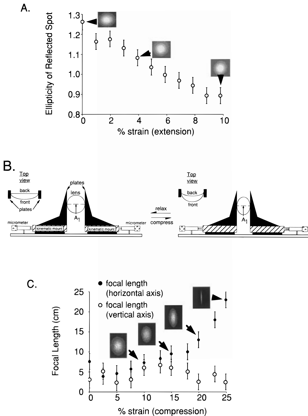
Figure 6. (a) Ellipticity of a laser beam that was reflected from the surface of an elastomeric mirror could be controlled by stretching the mirror. The insets show images of the output spot from the mirror where the ellipticity of the spot is >1 (elliptical spot, major axis in horizontal plane), \sim 1 (circular spot), and <1 (elliptical spot, major axis in vertical plane). These images were taken at a distance of \sim 6 cm from the front of the mirror. (b) Schematic of the jig used to test the performance of elastomeric lenses. The lens was held (by pressure) between aluminum plates attached to kinematic mounts. The mounts were equipped with micrometer screws; turning the micrometer screws in the appropriate direction either compressed the lens or allowed the lens to relax. Compressing the lens changed the curvature of the lens along the axis ( A_1 ) in which it was compressed ("top view"). Typically the lenses were \sim 1 – 2 cm in diameter (uncompressed). Drawing is not to scale. (c) Compressing an elastomeric lens along one axis ( A_1 , Figure 6b) increased the focal length of the lens along that axis. The lens was not compressed in the axis perpendicular to A_1 , and the focal length in that direction did not change (within the error of our measurement).
