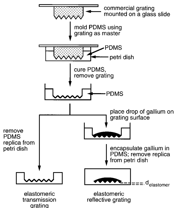
Figure 2. Schematic of the procedure for the fabrication of deformable gratings. Features are not drawn to scale. See text for details.
