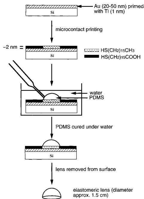
Figure 4. Schematic of the procedure for fabricating deformable elastomeric lenses. Microcontact printing formed a patterned SAM with hydrophobic and hydrophilic regions. A hydrophobic, liquid polymer (poly(dimethylsiloxane), PDMS) was delivered with a pipet to the surface of the patterned SAM, while the SAM was submerged in water. The PDMS spontaneously assembled on the hydrophobic regions in the shape of a lens. The PDMS was cured by heating and removed from the surface of the SAM. Features are not drawn to scale.
